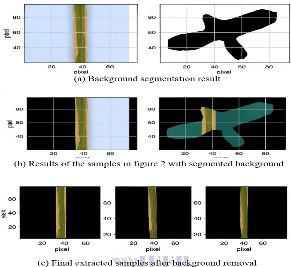
Figure 4: Images of the segmentation process
