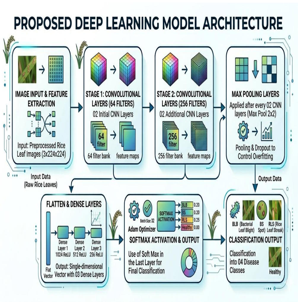
Figure 5: Proposed model architecture
