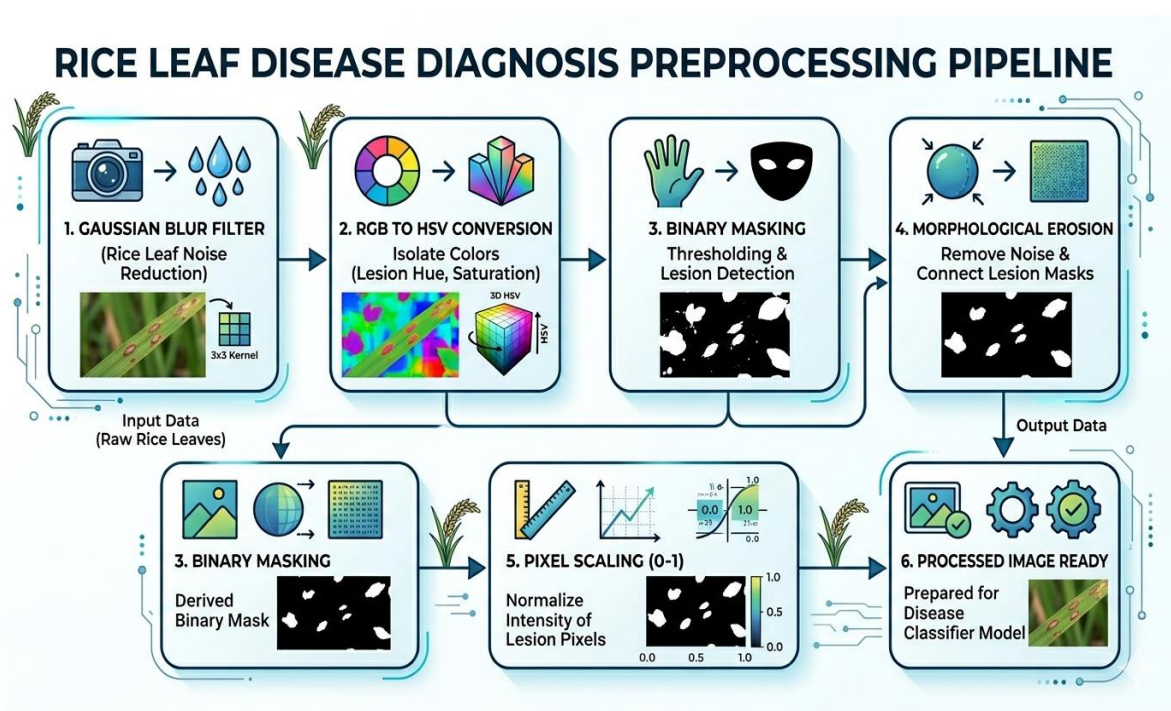
Figure 3: Rice leaf data preprocessing
