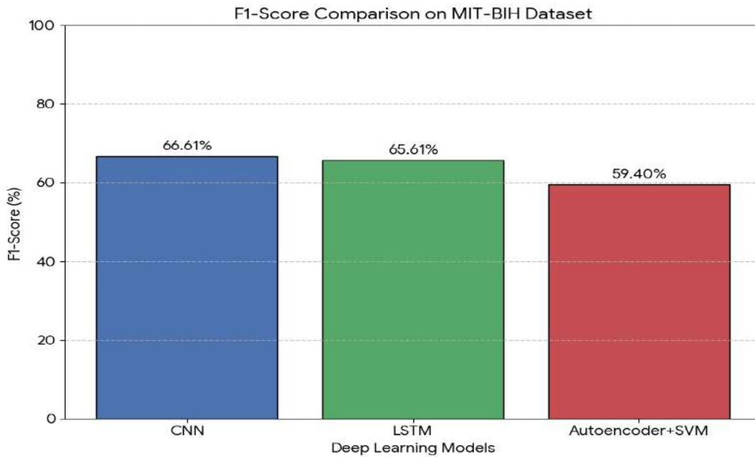
Figure 13. F1-Score MIT-BIH Dataset
