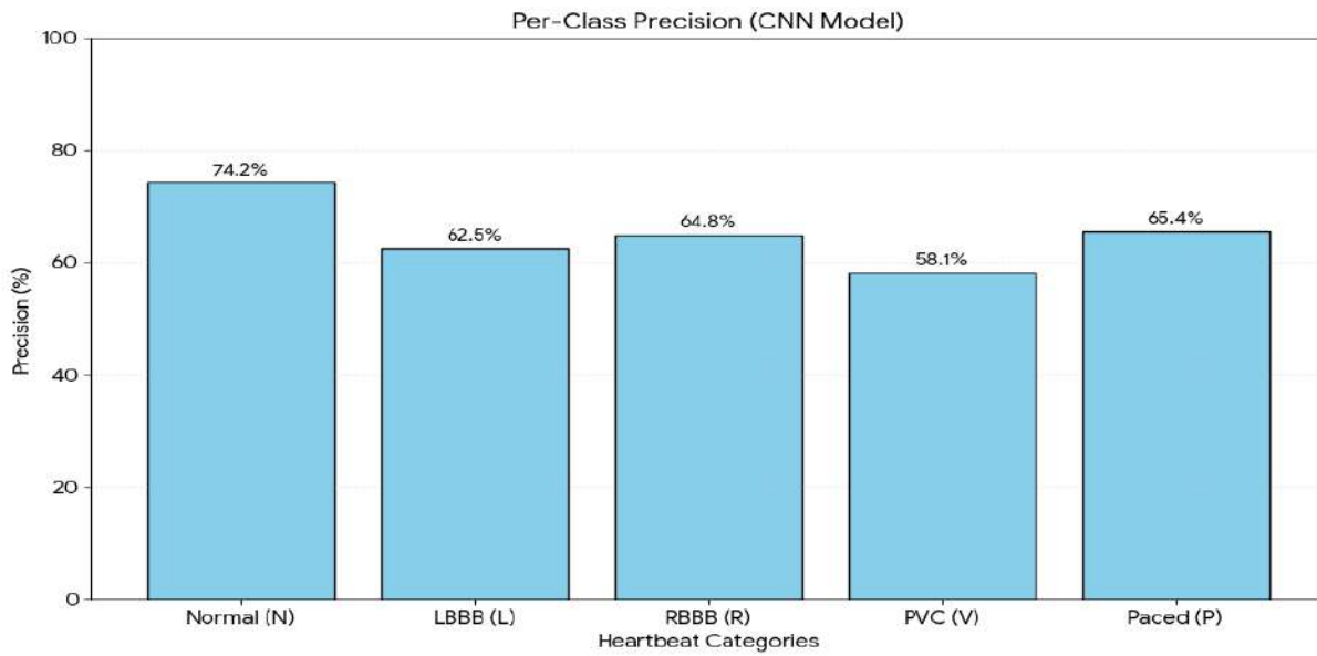
Figure 8. Precision CNN Model
