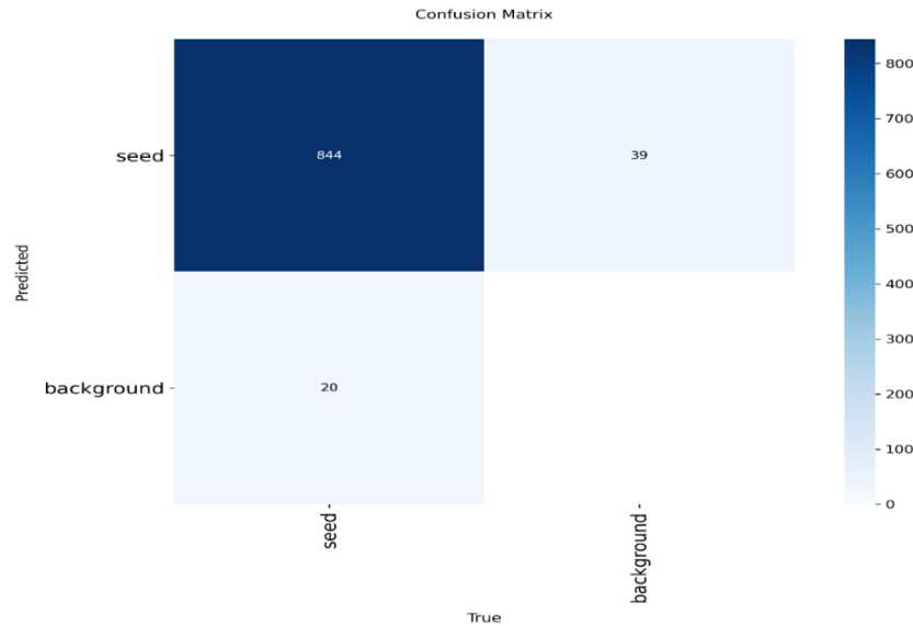
Figure 6. Confusion matrix of the YOLOv8n model on the canola seed validation dataset
