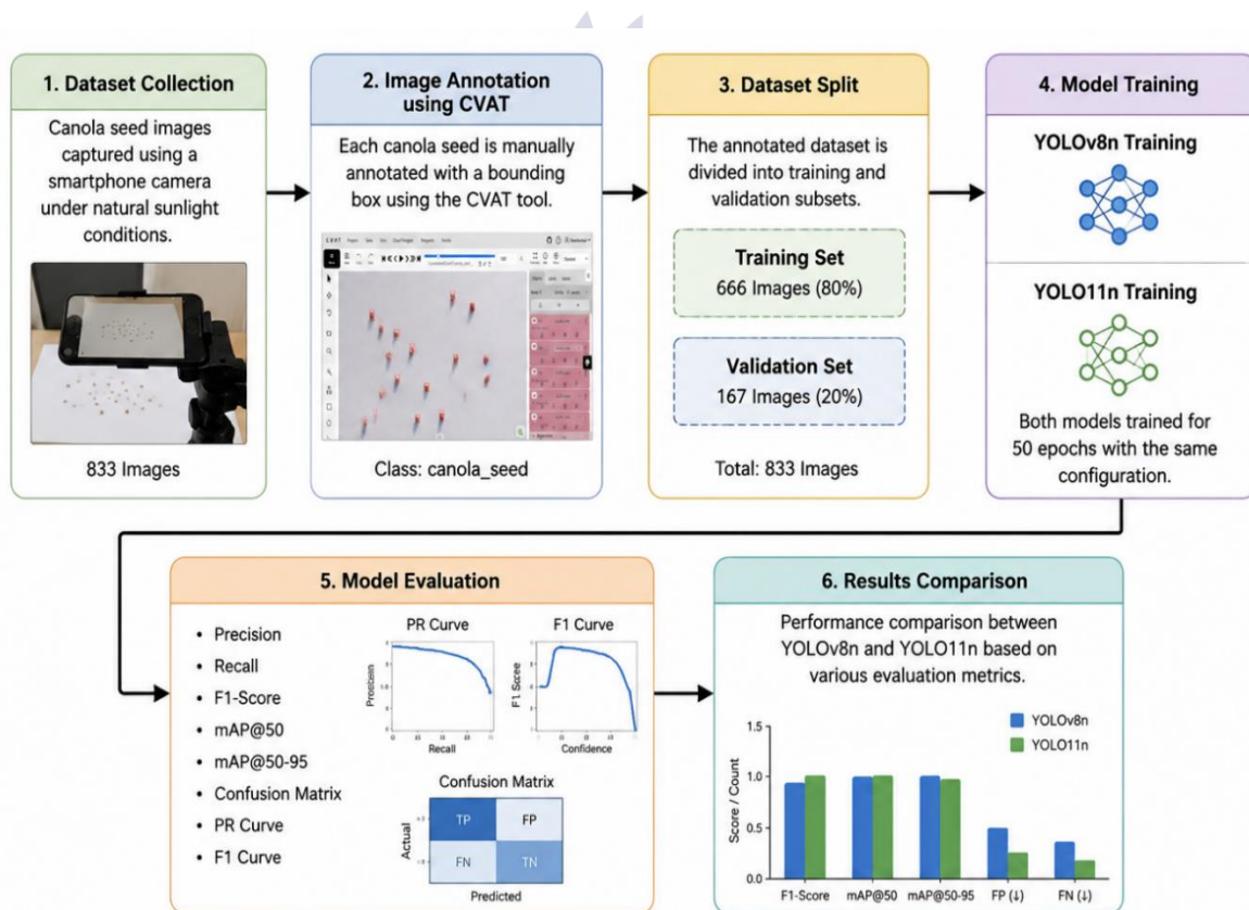
Figure 2. Overall workflow of the proposed canola seed detection and counting framework using YOLOv8n and YOLO11n.
